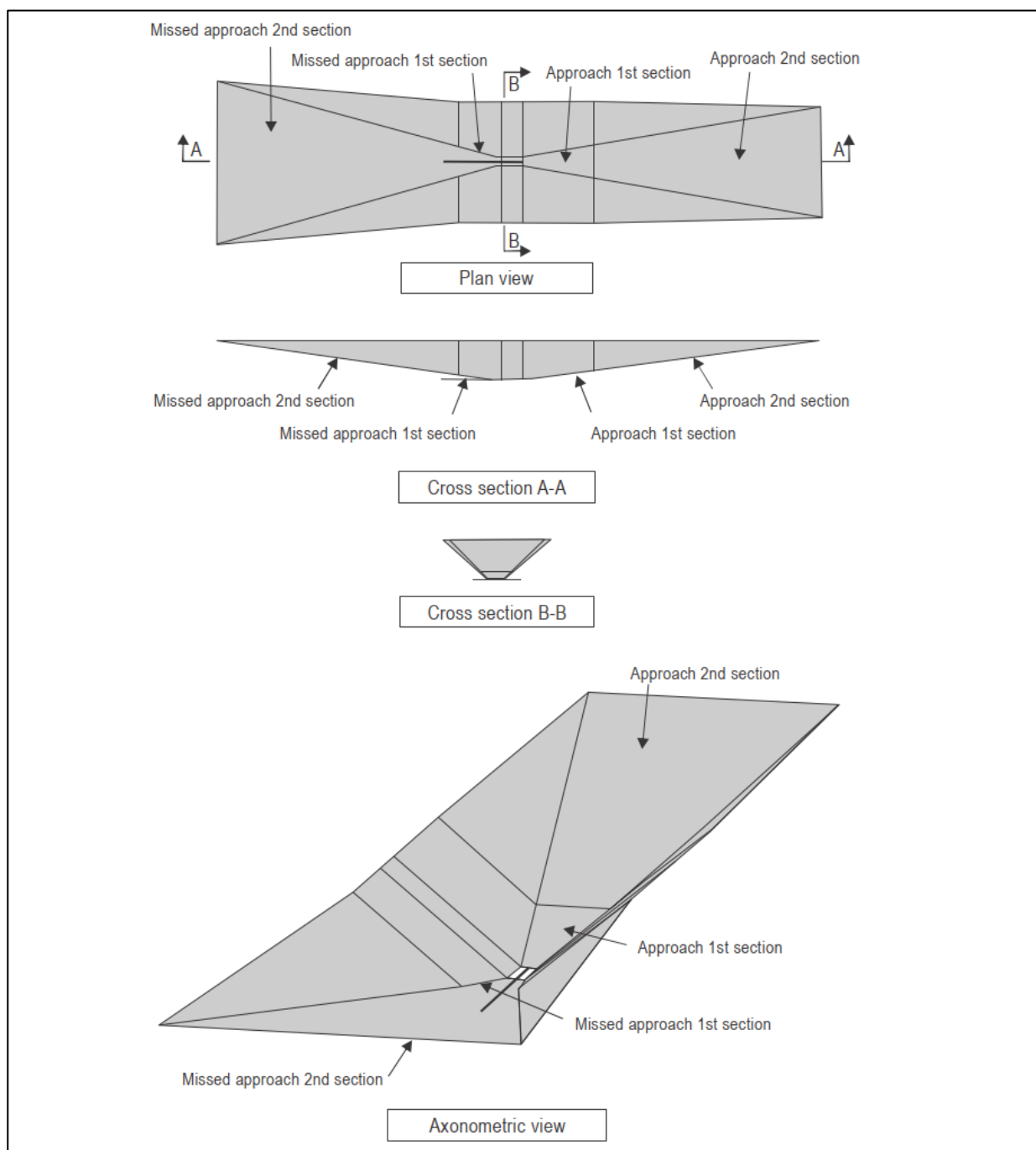
Figure D-6. Surface for precision approaches
