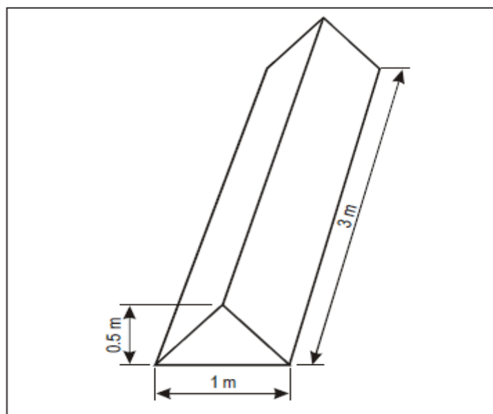
Figure E-34. Boundary markers
