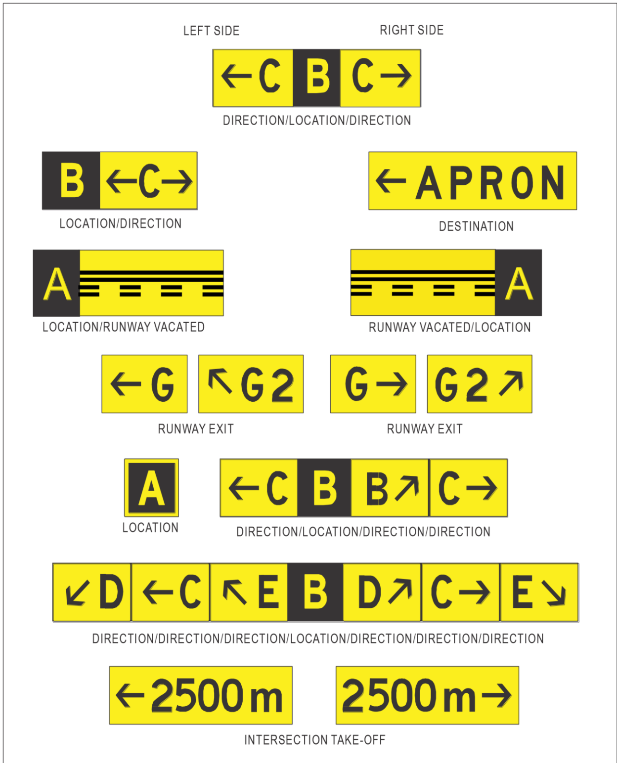
Figure E-31. Information signs
