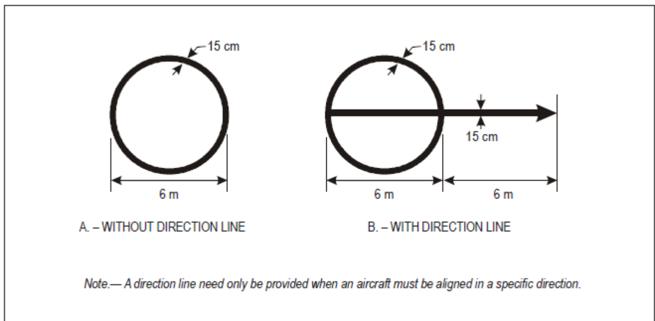
Figure E-9. VOR aerodrome checkpoint marking
