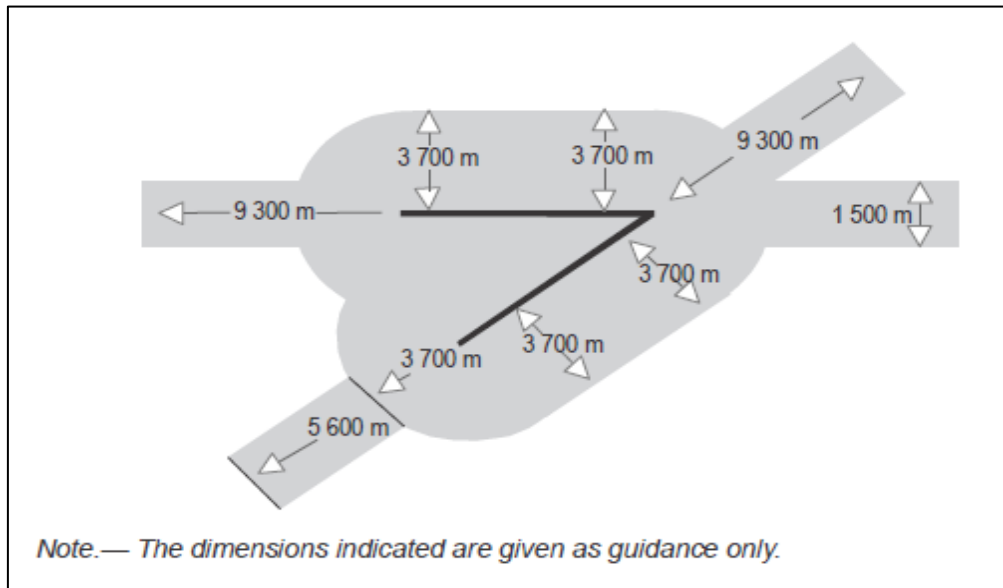
Figure E-12. Multiple runway laser-beam free flight zone
