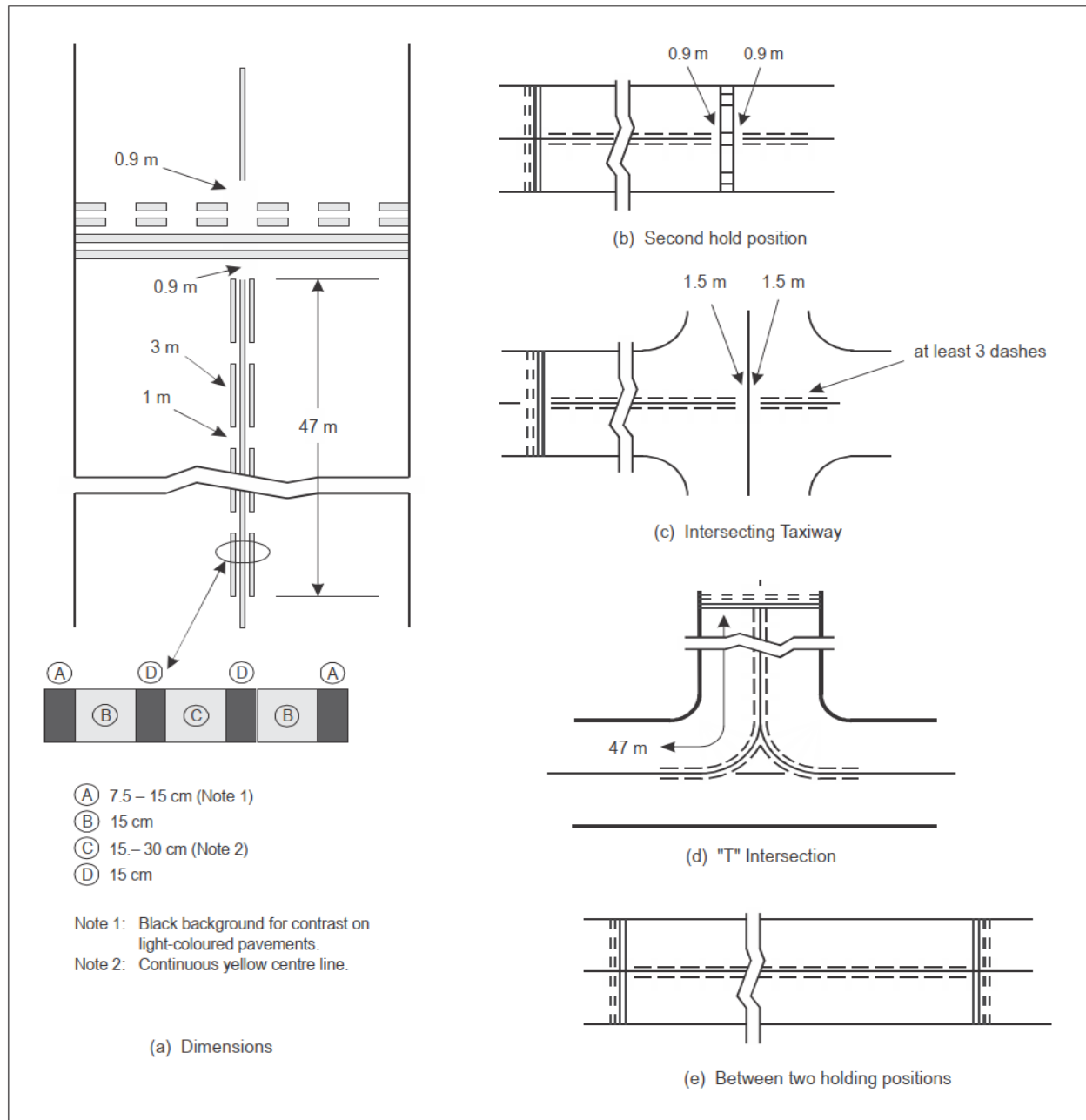
Figure E-7. Enhanced taxiway centre line marking
