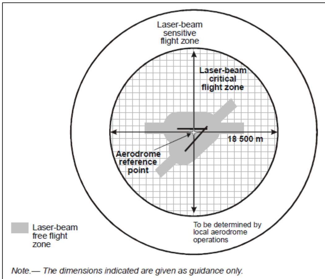
Figure E-11. Protected flight zones
