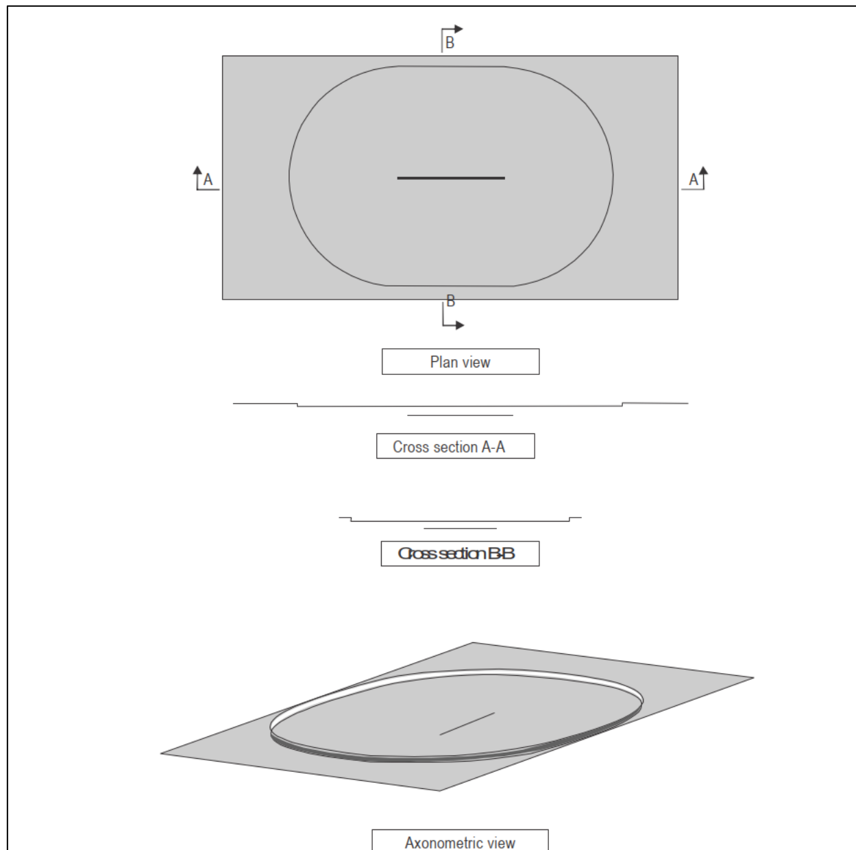
Figure D-5. Surface for straight-in instrument approaches
