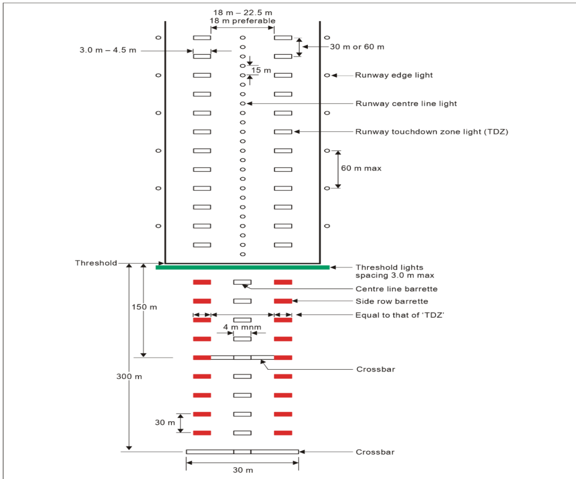
Figure E-14. Inner 300 m approach and runway lighting for precision approach runways, categories II and III
