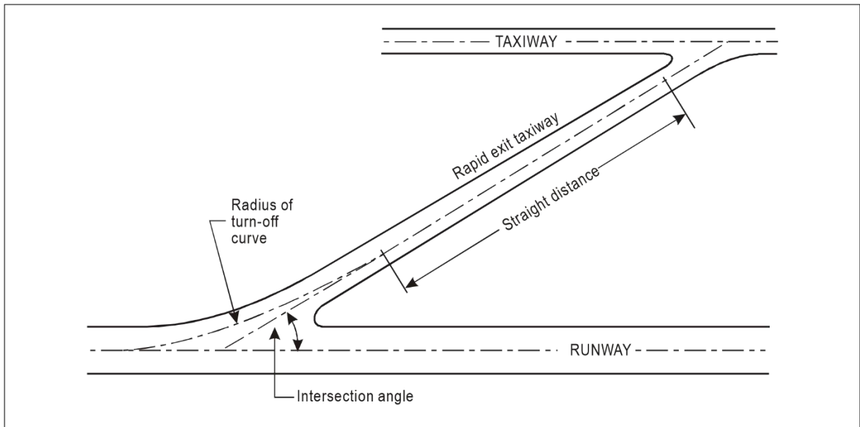
Figure C-3. Rapid exit taxiway
