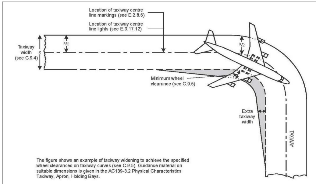
Figure C-2. Taxiway curve
