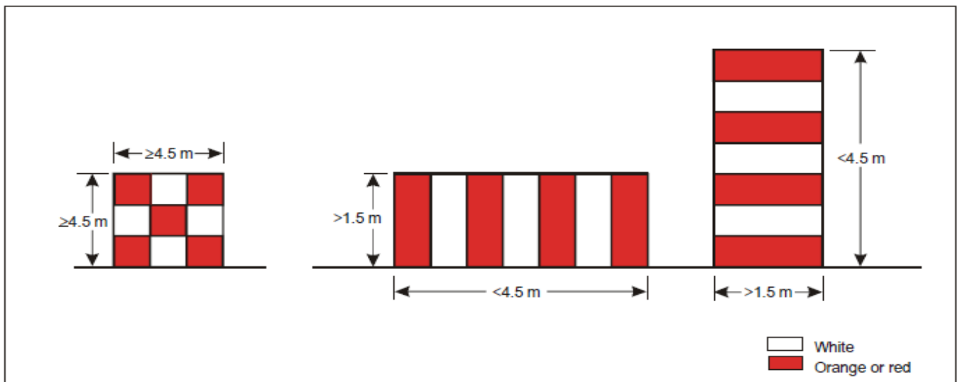
Figure F-1. Basic marking patterns
