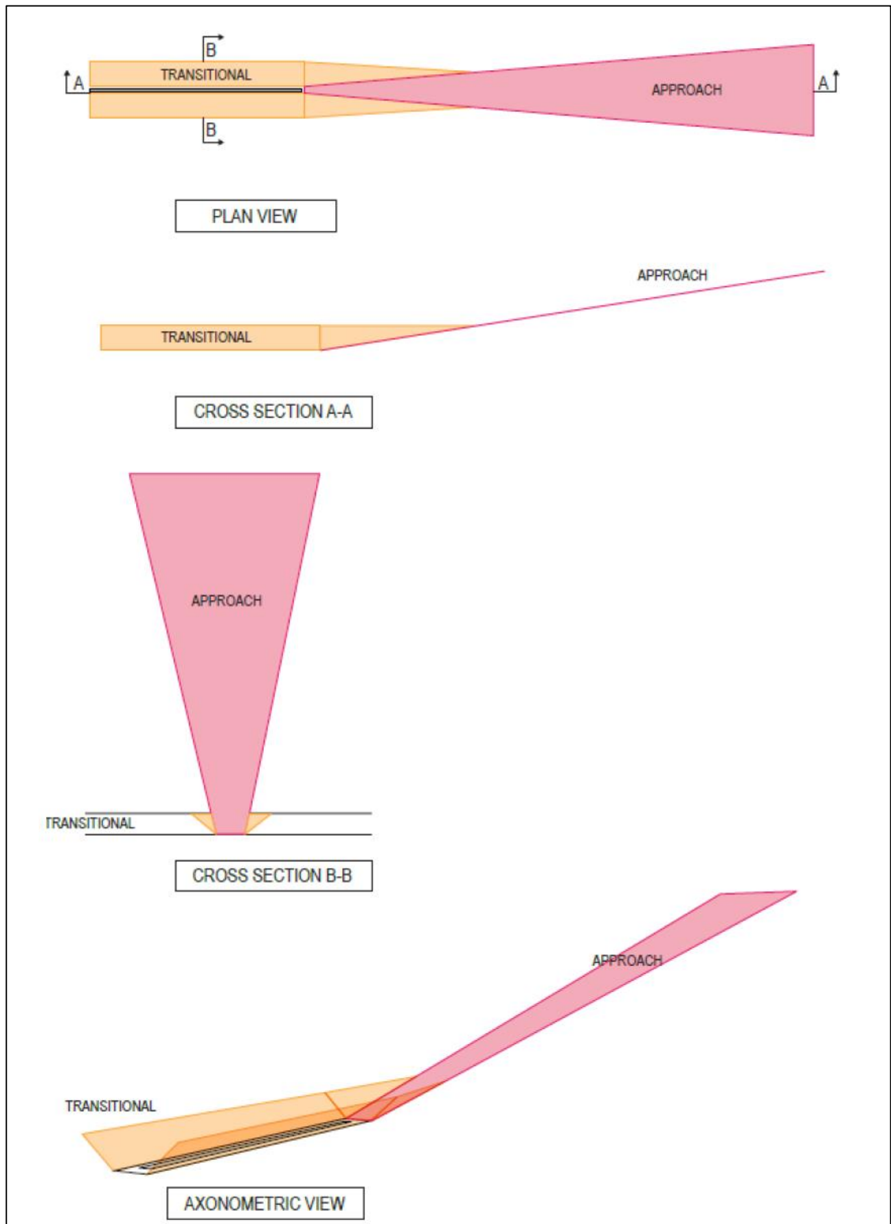
Figure D-1. Approach surface and transitional surfaces
