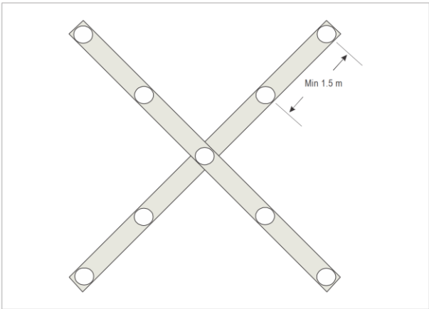
Figure G-2. Example of equivalent elevated closed runway lighting with five lights per branch
